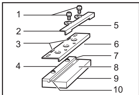
► 1. Pan head screw 2. Adjusting plate 3. Planer blade locating lugs 4. Gauge plate 5. Heel of adjusting plate 6. Set plate 7. Inside flank of gauge plate
